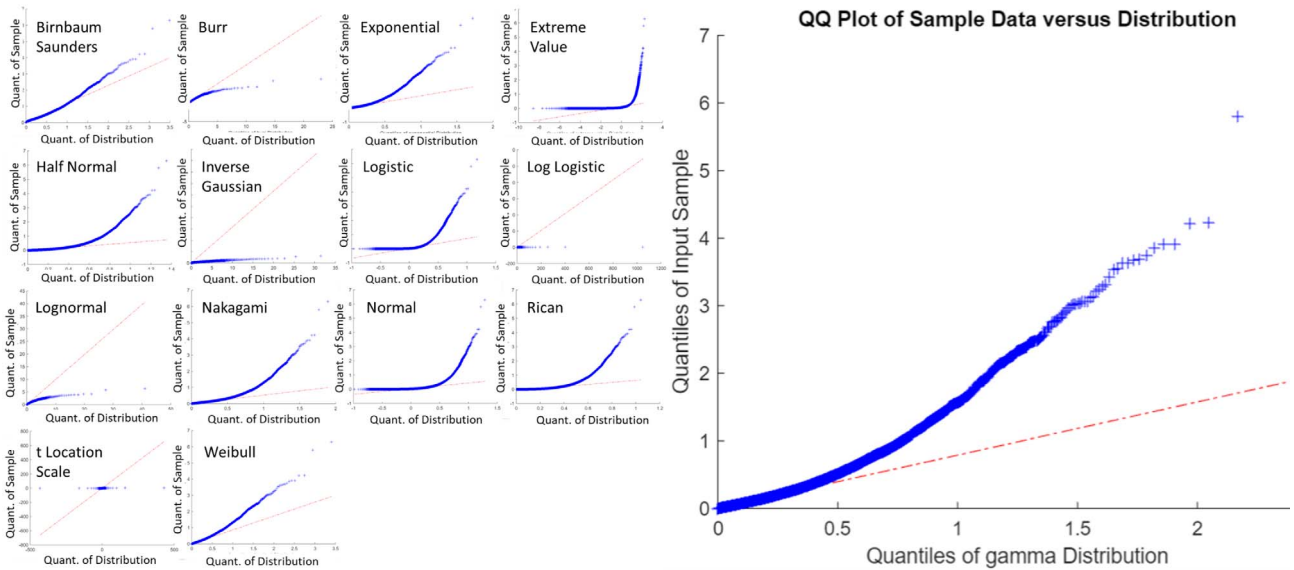
Figure 1. Quantile-quantile (QQ) plots for |\text{Grad\_Ne@100km}| in the polar region when different distributions are trialed to represent these data. The distributions trialed were: First row, left to right: Birnbaum Saunders, Burr, Exponential and Extreme Value. Second row, left to right: Half normal, Inverse Gaussian, Logistic and Loglogistic. Third row, left to right: Lognormal, Nakagami, Normal and Rician. Fourth row, left to right: tLocation Scale and Weibull distributions. Right-hand panel: Gamma.
