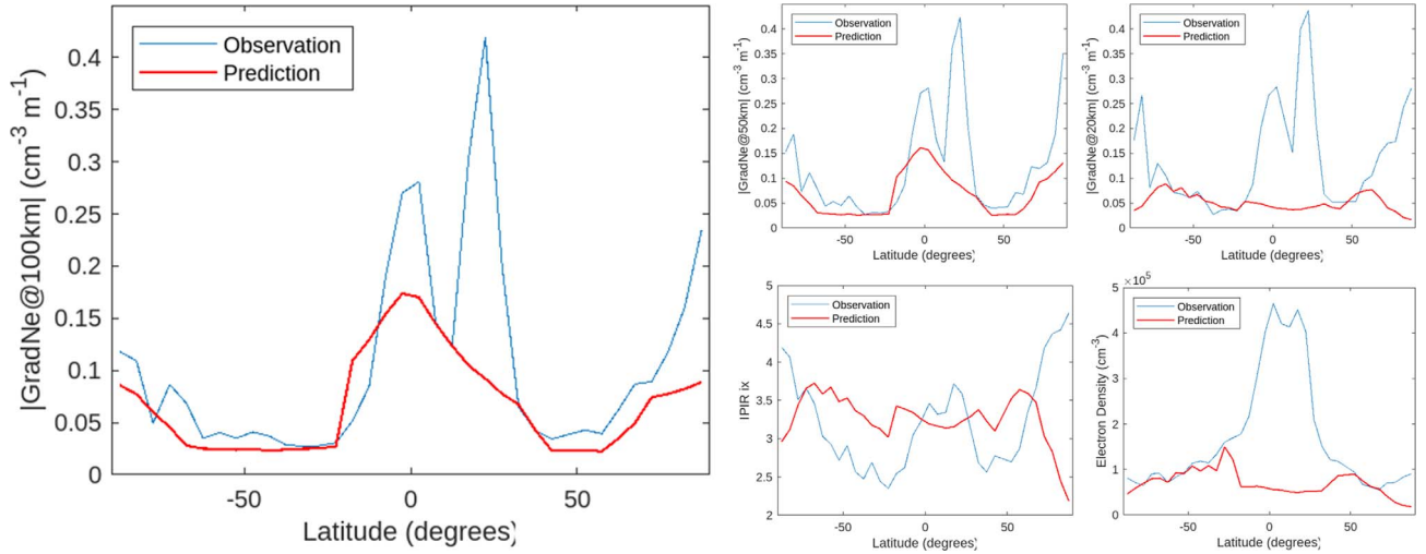
Figure 4. A statistical comparison between observations and predictions from the Swarm-VIP models in the 0°–15° geographic longitude sector for |\text{Grad\_Ne@100km}| (left panel), |\text{Grad\_Ne@50km}| (upper middle panel), |\text{Grad\_Ne@20km}| (upper right panel), the IPIR index (lower middle panel) and the electron density (lower right panel) as a function of latitude. This comparison shows average values in bins spanning 5° of latitude. Negative values of latitude indicate the southern hemisphere. Observations are indicated by the blue lines and predictions by the red lines.
