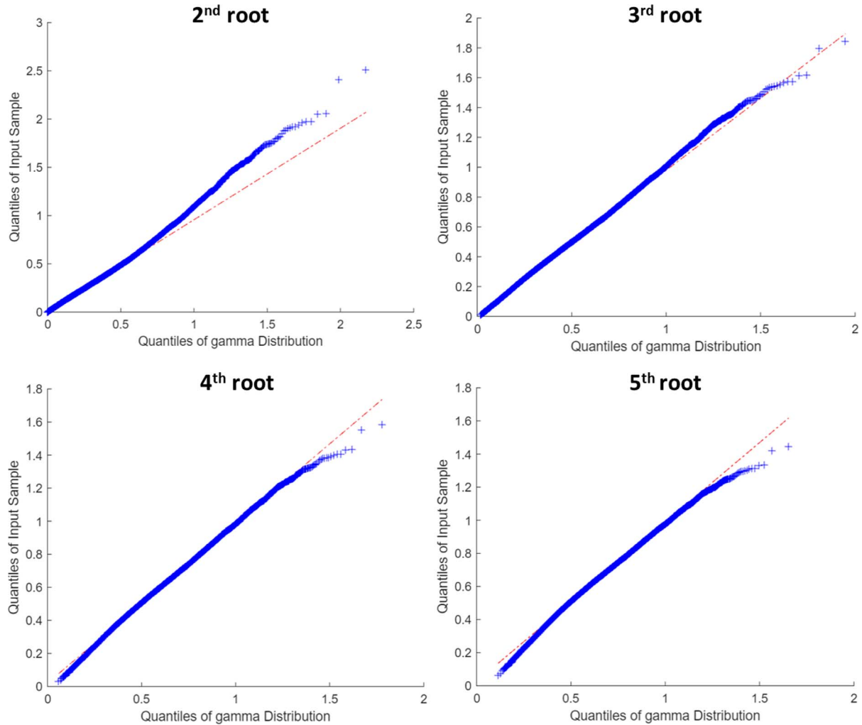
Figure 2. Quantile-quantile (QQ) plots for |\text{Grad\_Ne@100km}| in the polar region assuming a Gamma distribution when different transformations are trialled to these data. The transformations are 2nd root (upper left panel), 3rd root (upper right panel), 4th root (lower left panel) and 5th root (lower right panel).
